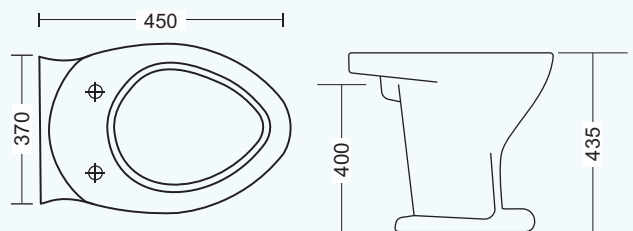
GI-406 RAILWAY WATER CLOSET (HOPPER) L 450 W 370 H 435mm
