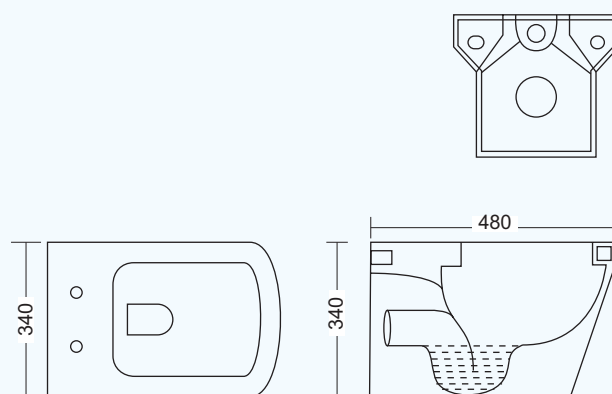
GI-302 RAGA WALL HUNG
