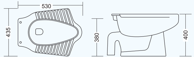
GI-404 ANGLO INDIAN WATER CLOSET L 530 W 435 H 400mm S Trap
