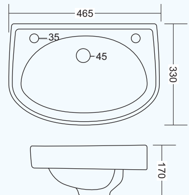
GI-608 VENUE BANTAM ROUND 18" x 12" ROUND WASH BASIN
