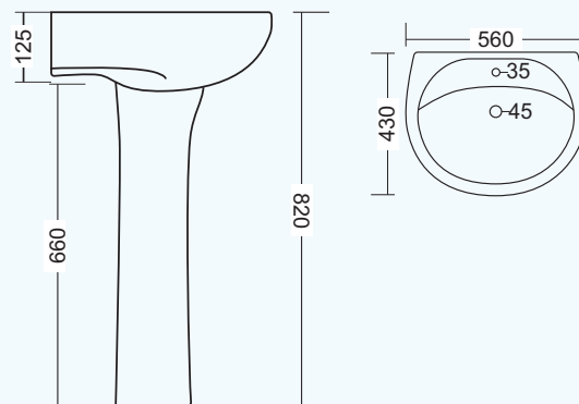
GI-501 CUBA 22" x 16" REPOSE SET L 430 W 560 H 820mm
