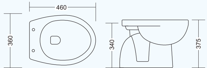
GI-405 CONCEALED WATER CLOSET L 460 W 360 H 375mm S Trap
