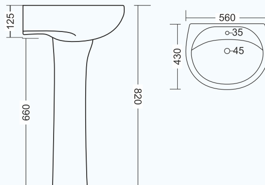
GI-501 CUBA 22" x 16" REPOSE SET
