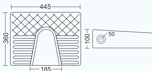
GI-410 | LADIES URINAL L 360 W 445 H 100mm
