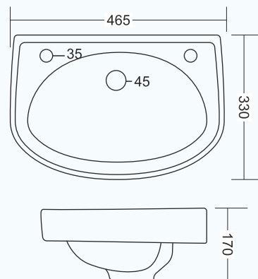
GI-608 VENUE BANTAM ROUND 18" x 12" ROUND WASH BASIN
